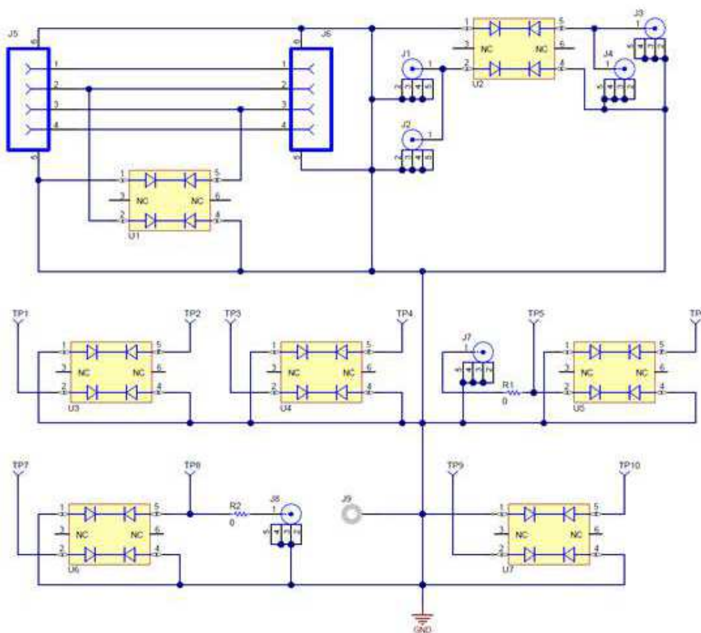
Figure 5. TPD2E1B06DRLEVM Schematic
