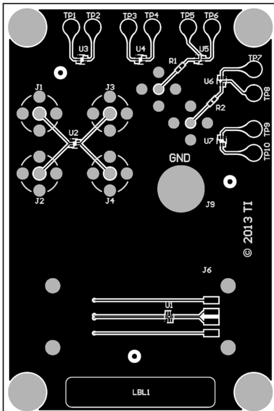
Figure 3. TPD2E1B06DRLEVMM Top Layer
